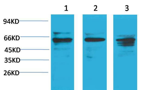
Western blot analysis of 1) HeLa, 2)3T3, 3) PC12 with Akt1 Rabbit pAb diluted at 1:2,000.
