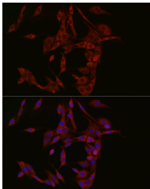
Immunofluorescence analysis of PC-12 cells using cGAS Rabbit MAb at dilution of 1:50 (40x lens). Blue: DAPI for nuclear staining.
