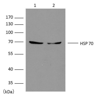
Western blot analysis of extracts from Hela (Lane 1)MCF-7 (Lane 2) using HSP70 diluted at 1:2000.
