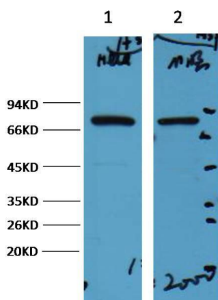
Western blot analysis of Hela 2i Mouse Brain with HSP70 mAb diluted at:2000
