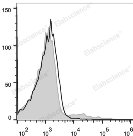
Human peripheral blood lymphocytes are stained with PE/Cyanine5 Anti-Human IgM Antibody (filled gray histogram) or Mouse IgG1 Isotype Control PE/Cyanine5 (empty black histogram).
