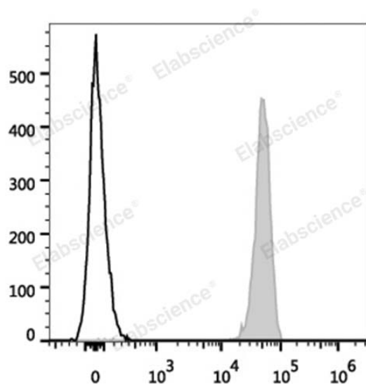
Human platelets are stained with PerCP/Cyanine5.5 Anti-Human CD9 Antibody (filled gray histogram). Unstained platelets (empty black histogram) are used as control.
