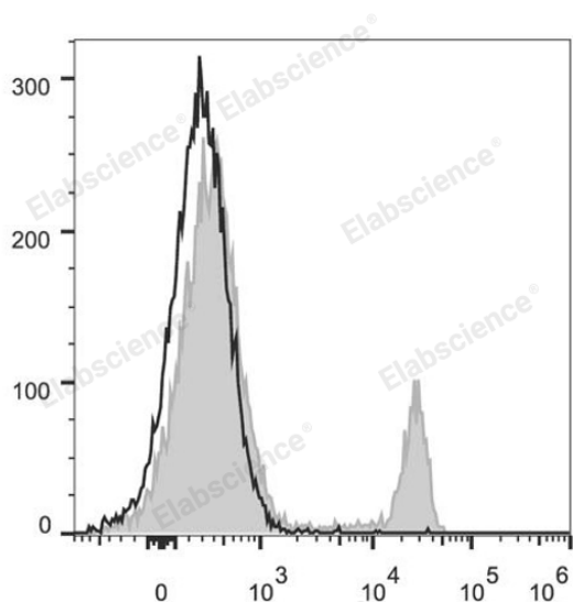
C57BL/6 murine splenocytes are stained with PerCP/Cyanine5.5 Anti-Mouse CD8a Antibody (filled gray histogram). Unstained splenocytes (empty black histogram) are used as control.
