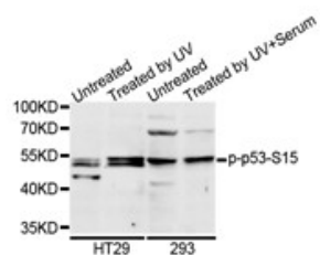
Western blot analysis of extracts of various cell lines, using Phospho-p53 (Ser15) antibody.
