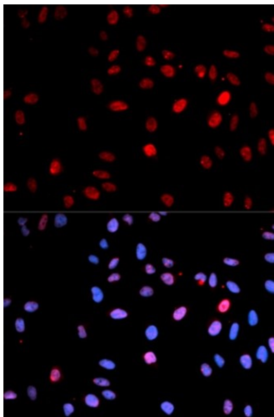
Immunofluorescence analysis of U2OS cell using Phospho-p53 (Ser15) antibody. Blue: DAPI for nuclear staining.
