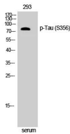
Western Blot analysis of NIH-3T3 cells using Phospho-Tau (S356) Polyclonal Antibody diluted at 1:500
