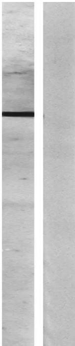
Western blot analysis of lysates from 293 cells treated with serum 10% 15', using Tau (Phospho-Ser356) Antibody. The lane on the right is blocked with the phospho peptide.
