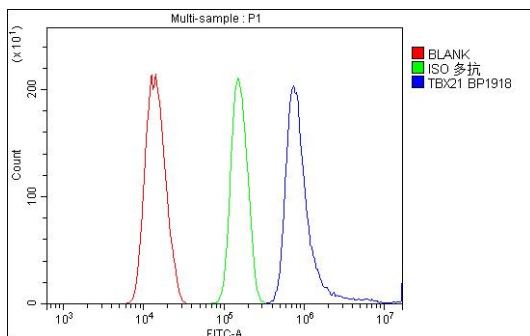
Figure 3. Flow Cytometry analysis of NRK cells using anti-TBX21 antibody. Overlay histogram showing NRK cells stained with (Blue line).The cells were blocked with 10% normal goat serum. And then incubated with rabbit anti-TBX21 Antibody (1mug/1x10 6 cells) for 30 min at 20°C. DyLight®488 conjugated goat anti-rabbit IgG (5-10mug/1x10 6 cells) was used as secondary antibody for 30 minutes at 20°C. Isotype control antibody (Green line) was rabbit IgG (1mug/1x10 6 ) used under the same conditions. Unlabelled sample (Red line) was also used as a control.
