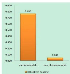
Enzyme-Linked Immunosorbent Assay (Phospho-EUSA) for Immunogen Phosphopeptide (Phospho-left) and Non-Phosphopeptide (Phospho-right), using Vimentin (Phospho-Ser56) Antibody
