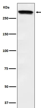
Western blot analysis of Huntingtin expression in HeLa cell lysate.
